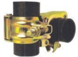
ISPC - JDC JAPANESE DOUBLE COUPLER FOR TUBE OD 48.3MM & 42.3MM (JIS : G3444 / SS-311)
